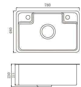
型号: ZP7848DW (压纹) 规格: 780x480x230mm 开孔尺寸: 750x450mm
