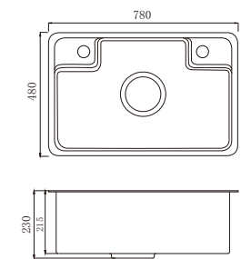
型号: ZP7848DH 规格: 780x480x230mm 开孔尺寸: 750x450mm
